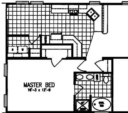
MASTER BEDROOM 1
